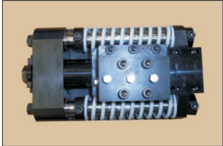
Spring Loaded out of round Tool Slide... cutoff and bevel
